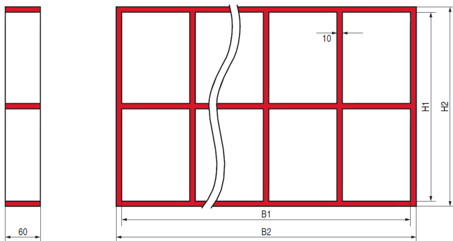
CFS-T SS multiple frames (double-row)
